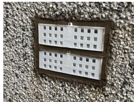
Photo showing Kitemark™ Certified Anti Flood Airbricks, in white
